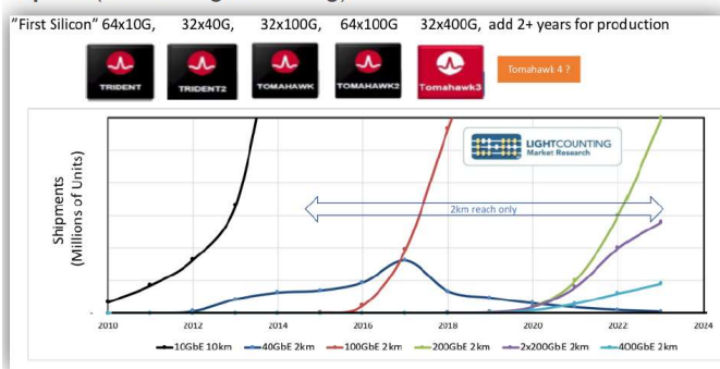
Correlation Between “First Switch Silicon” and Shipments of Optics (Source: LightCounting)
